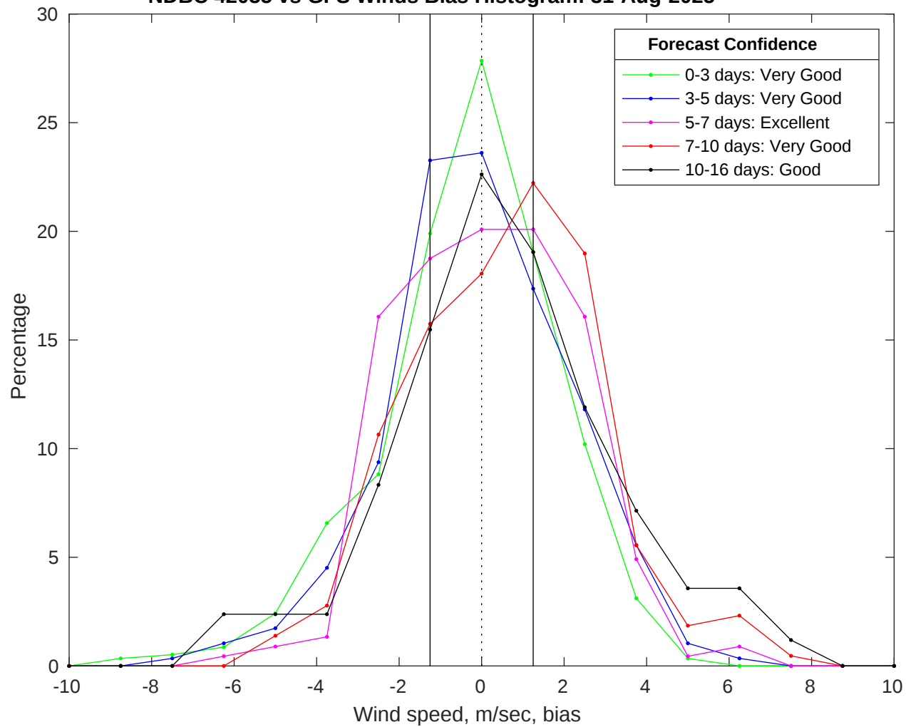
NDBC 42035 vs GFS Winds Bias Histogram: 31-Aug-2025
