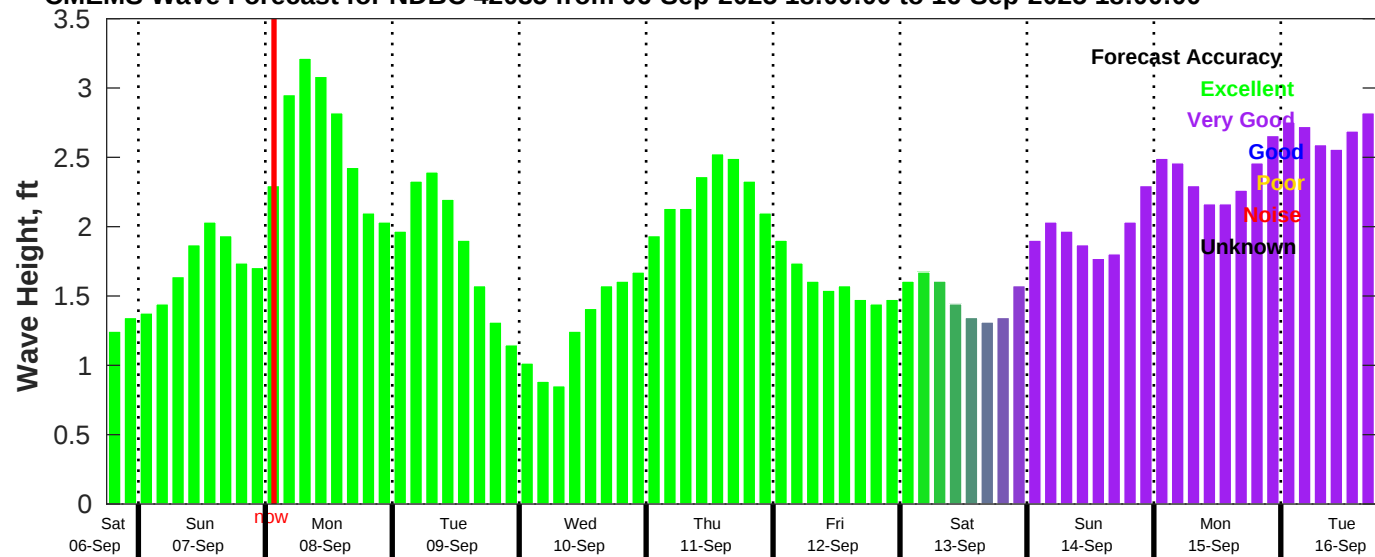
CMEMS Wave Forecast for NDBC 42035 from 06-Sep-2025 18:00:00 to 16-Sep-2025 18:00:00
