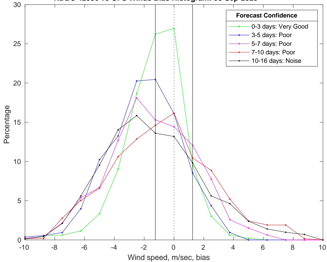
NDBC 42036 vs GFS Winds Bias Histogram: 08-Sep-2025
