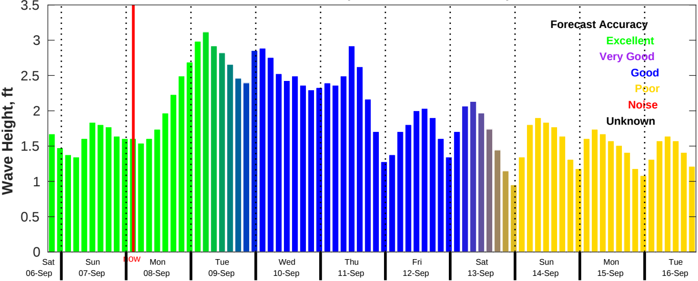
CMEMS Wave Forecast for NDBC 42036 from 06-Sep-2025 19:00:00 to 16-Sep-2025 19:00:00
