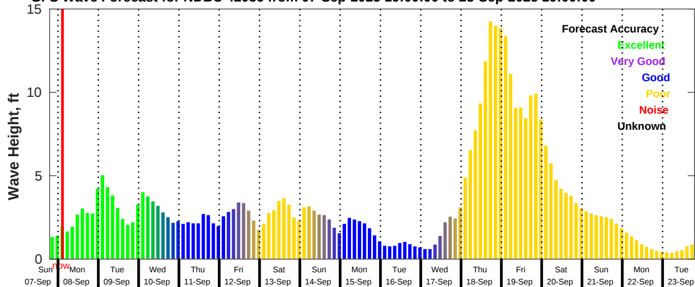
GFS Wave Forecast for NDBC 42036 from 07-Sep-2025 19:00:00 to 23-Sep-2025 19:00:00
