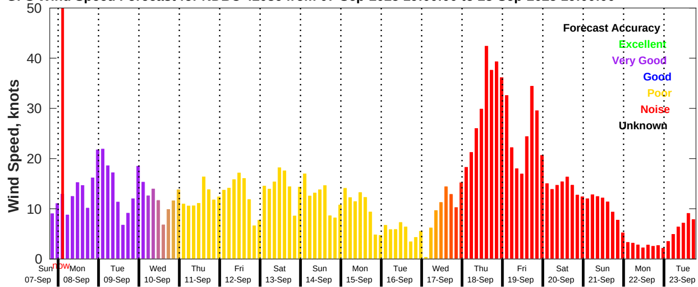
GFS Wind Speed Forecast for NDBC 42036 from 07-Sep-2025 19:00:00 to 23-Sep-2025 19:00:00
