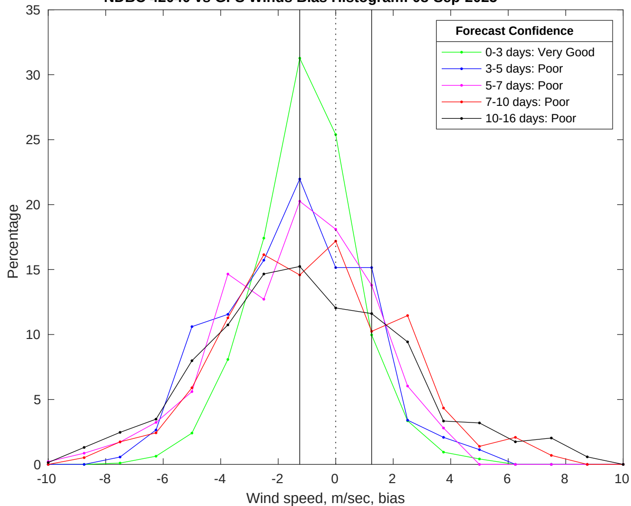
NDBC 42040 vs GFS Winds Bias Histogram: 08-Sep-2025
