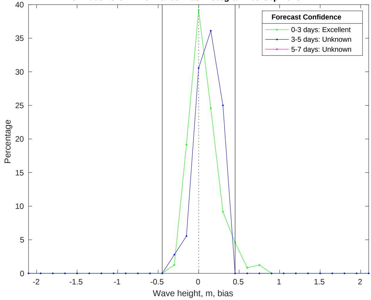
NDBC 44008 vs CMEMS Waves Bias Histogram: 08-Sep-2025
