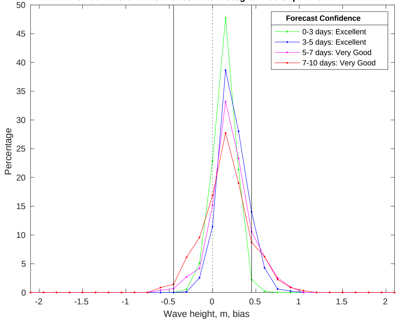
NDBC 46011 vs CMEMS Waves Bias Histogram: 08-Sep-2025
