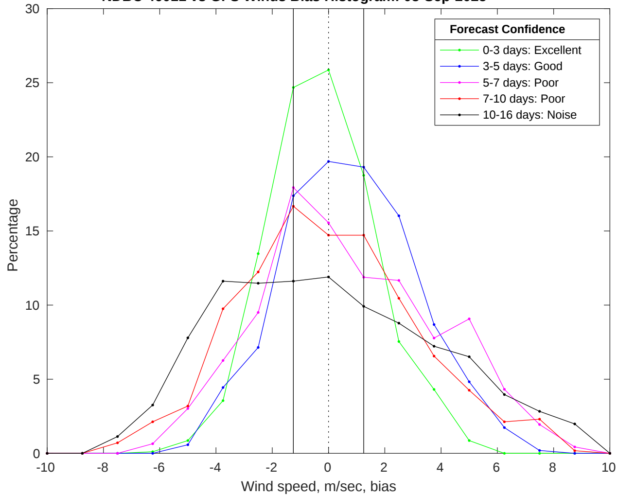
NDBC 46011 vs GFS Winds Bias Histogram: 08-Sep-2025
