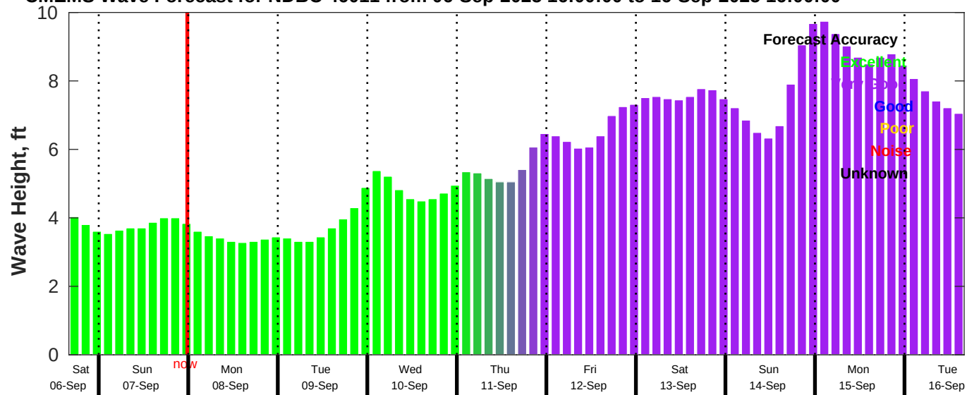
CMEMS Wave Forecast for NDBC 46011 from 06-Sep-2025 16:00:00 to 16-Sep-2025 16:00:00
