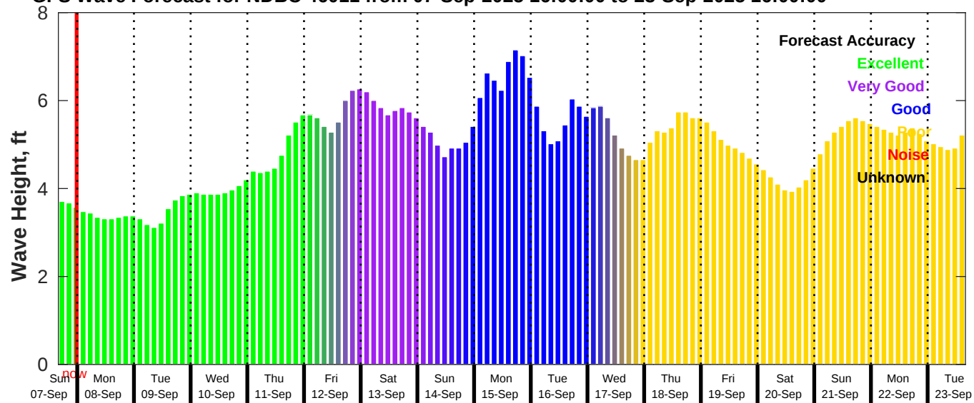
GFS Wave Forecast for NDBC 46011 from 07-Sep-2025 16:00:00 to 23-Sep-2025 16:00:00
