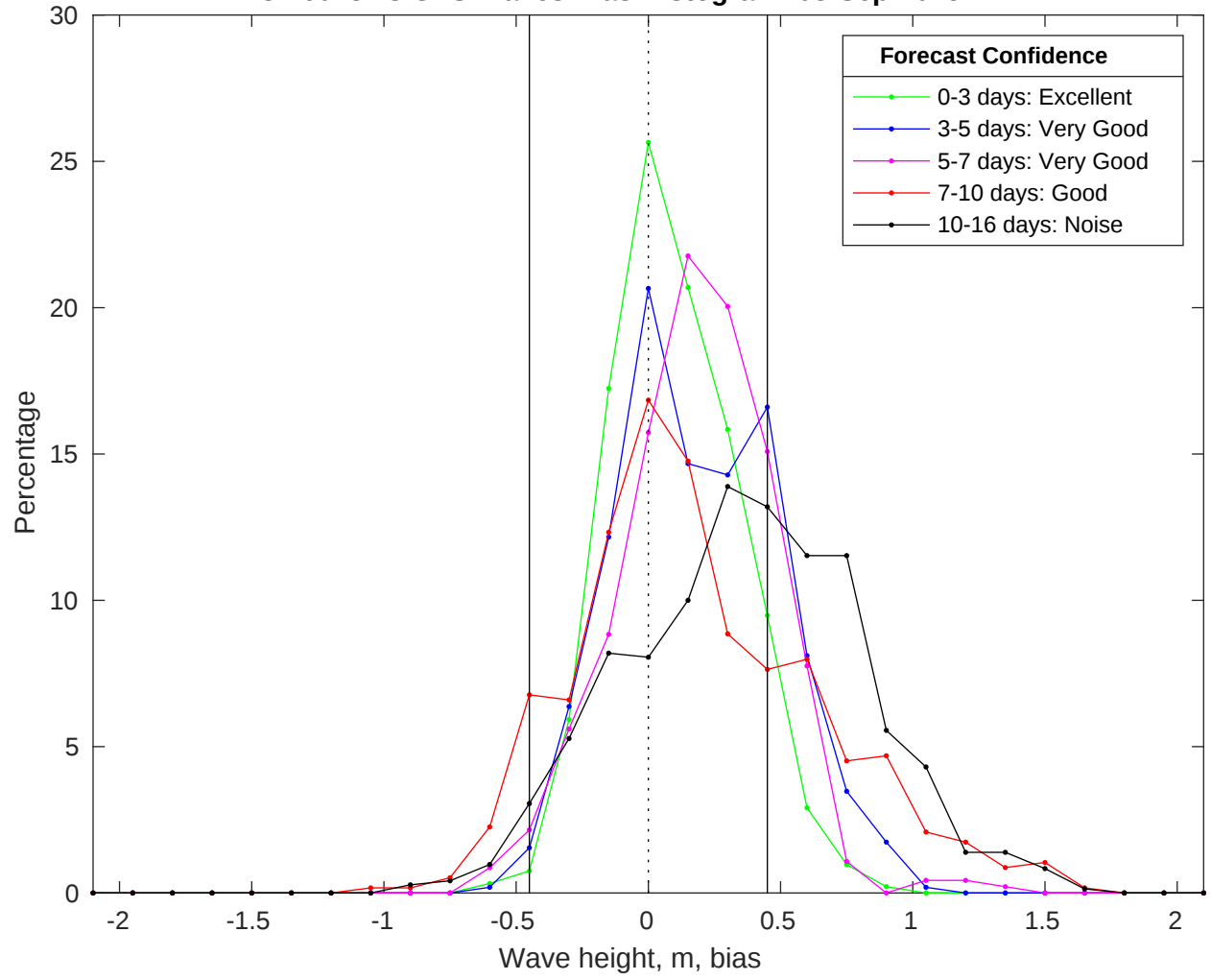
NDBC 46028 vs GFS Waves Bias Histogram: 08-Sep-2025
