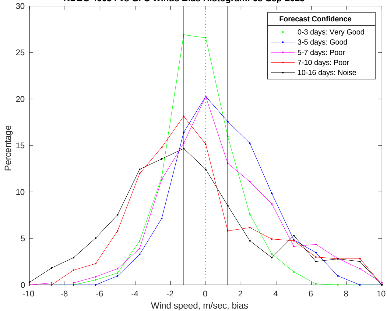
NDBC 46054 vs GFS Winds Bias Histogram: 08-Sep-2025
