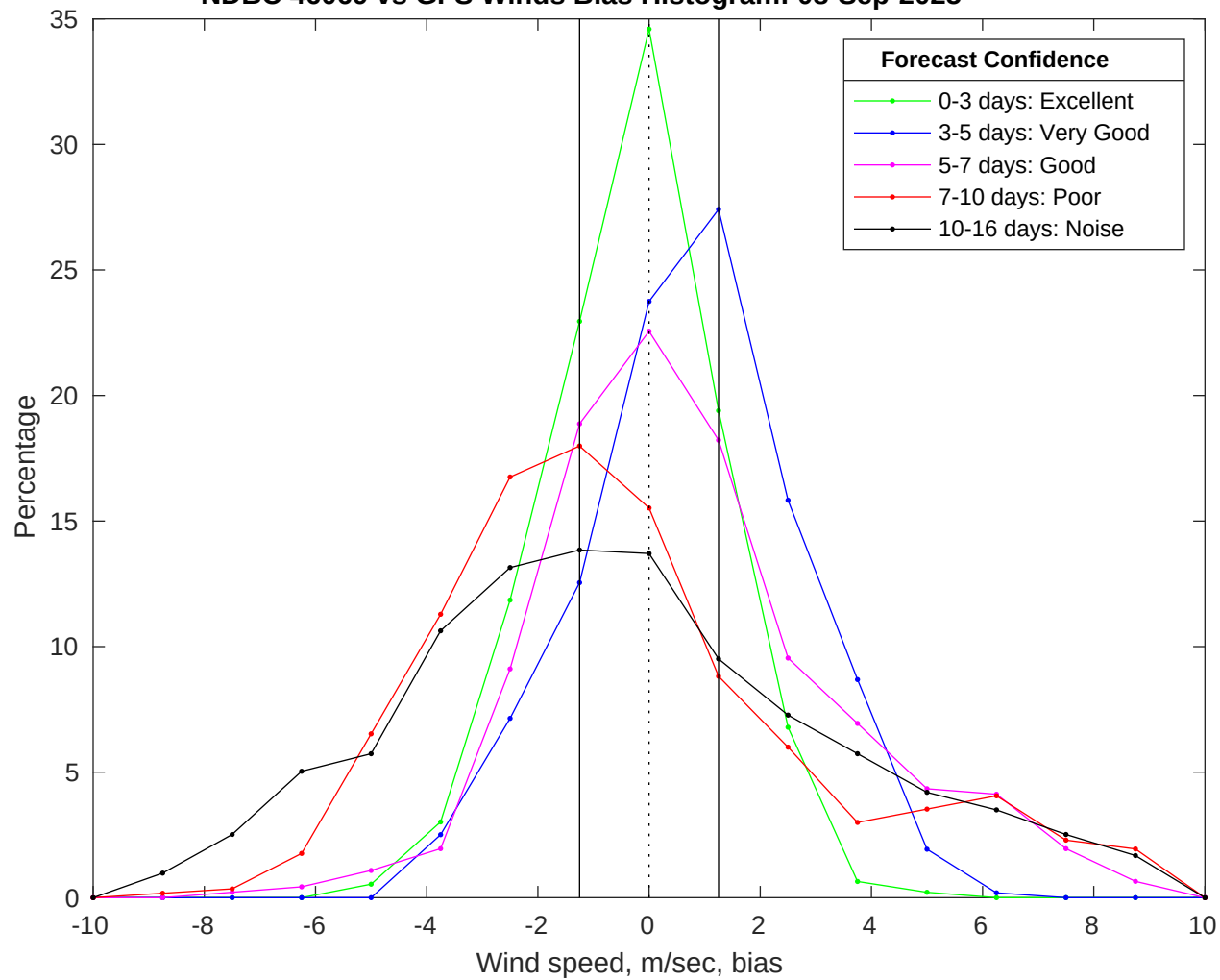
NDBC 46069 vs GFS Winds Bias Histogram: 08-Sep-2025
