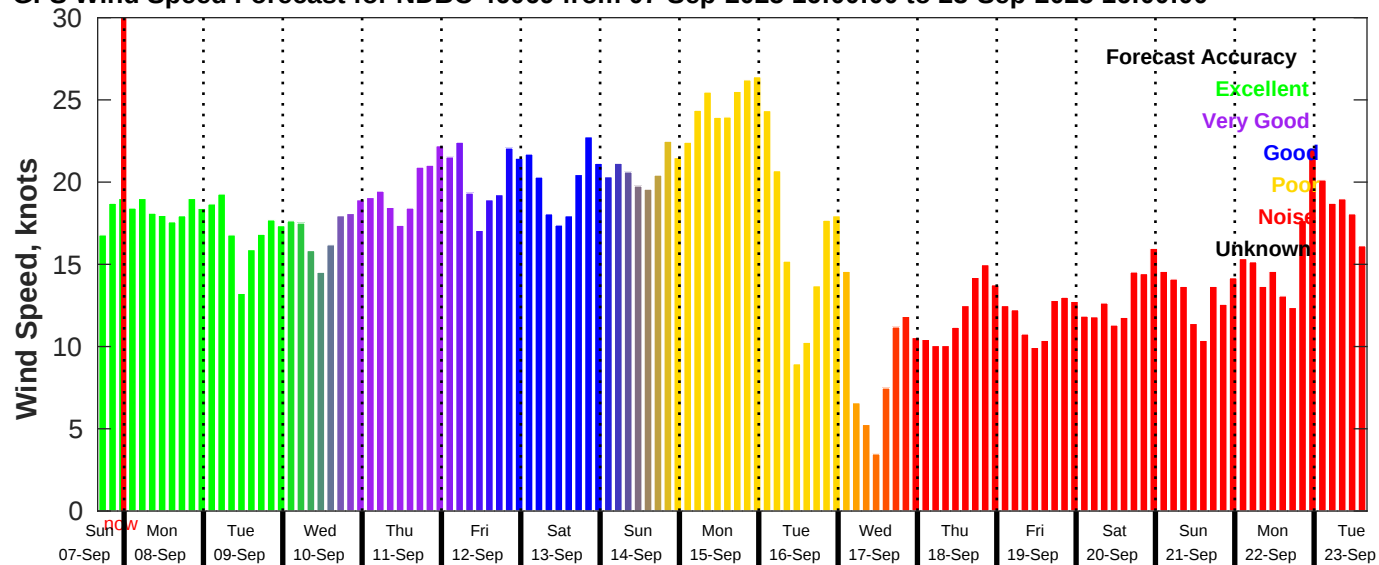
GFS Wind Speed Forecast for NDBC 46069 from 07-Sep-2025 16:00:00 to 23-Sep-2025 16:00:00
