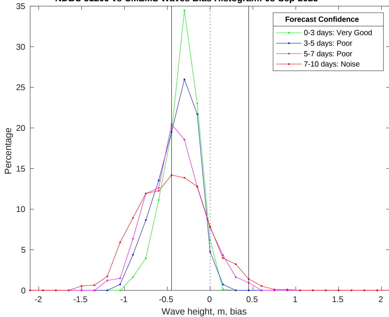
NDBC 51209 vs CMEMS Waves Bias Histogram: 08-Sep-2025
