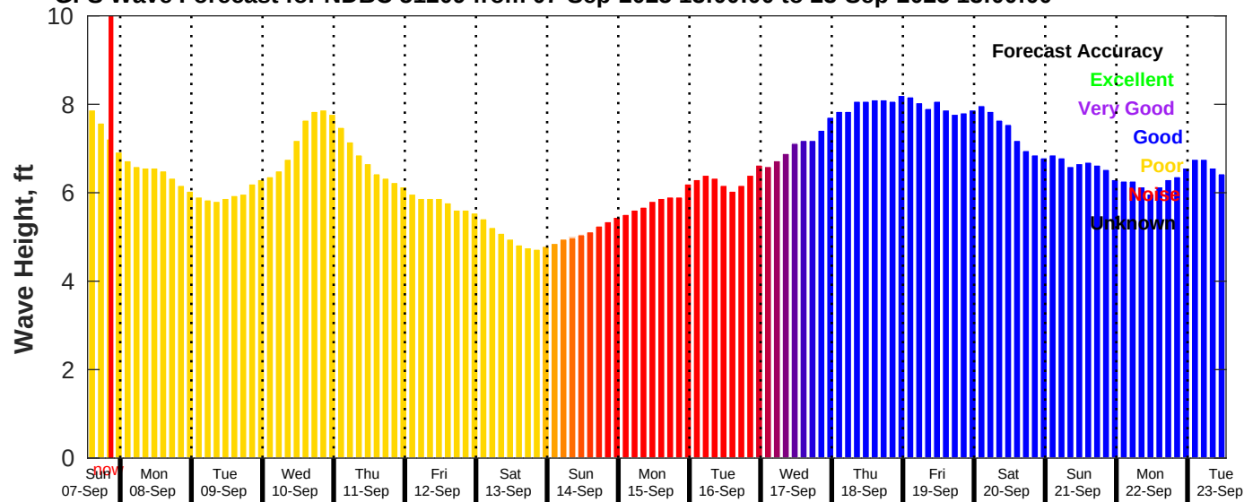
GFS Wave Forecast for NDBC 51209 from 07-Sep-2025 13:00:00 to 23-Sep-2025 13:00:00
