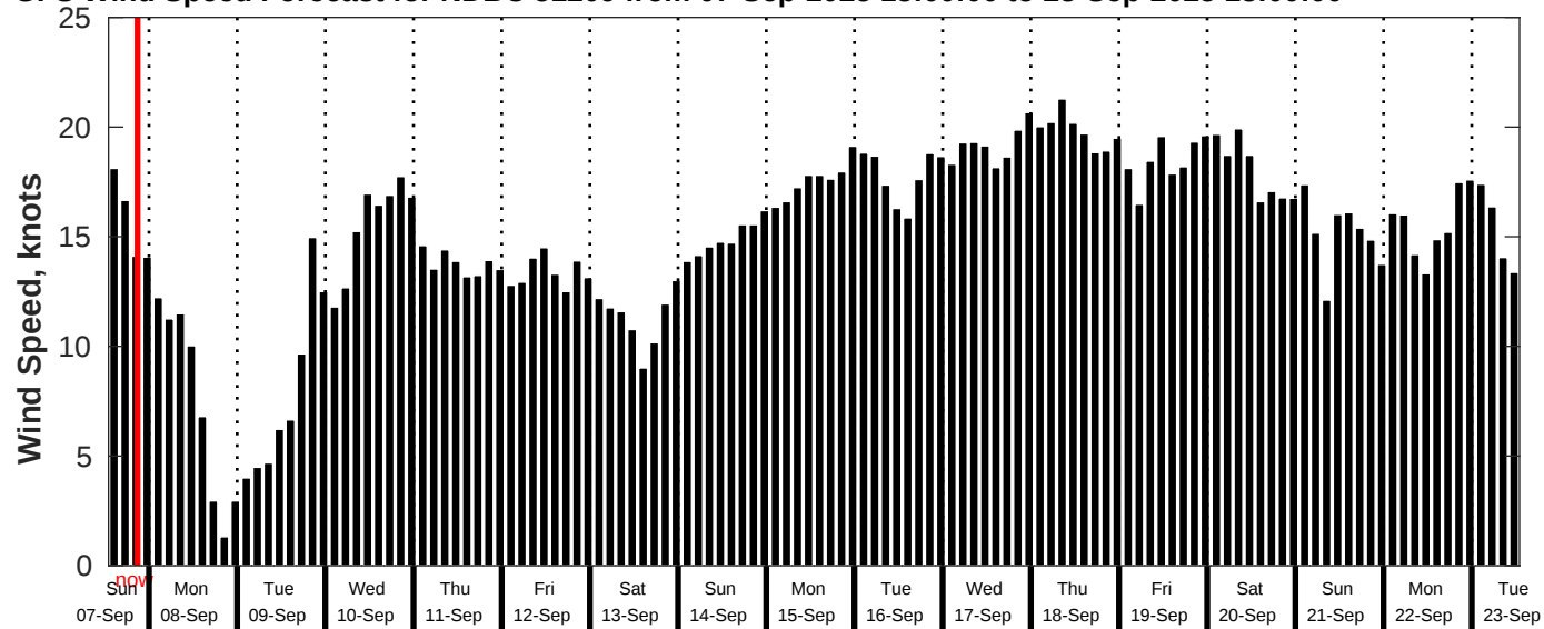
GFS Wind Speed Forecast for NDBC 51209 from 07-Sep-2025 13:00:00 to 23-Sep-2025 13:00:00
