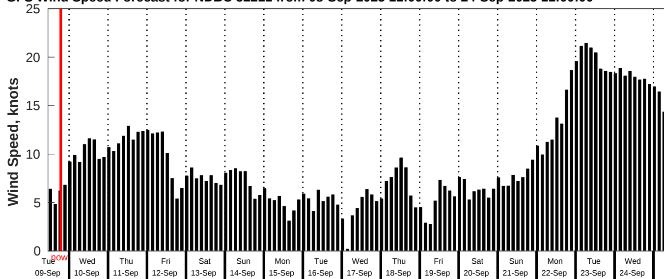
GFS Wind Speed Forecast for NDBC 52211 from 08-Sep-2025 11:00:00 to 24-Sep-2025 11:00:00
