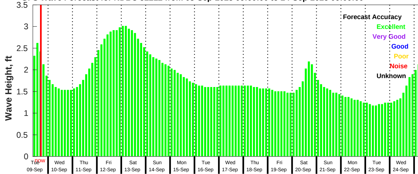
GFS Wave Forecast for NDBC 52212 from 08-Sep-2025 09:00:00 to 24-Sep-2025 09:00:00
