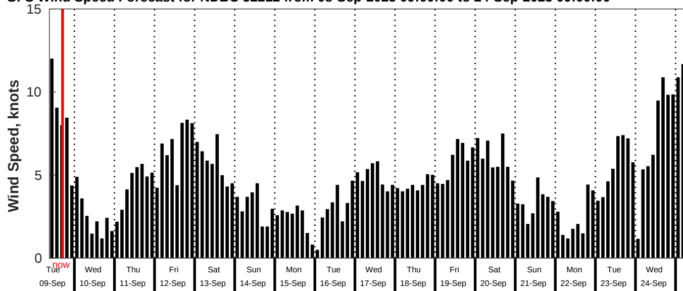
GFS Wind Speed Forecast for NDBC 52212 from 08-Sep-2025 09:00:00 to 24-Sep-2025 09:00:00
