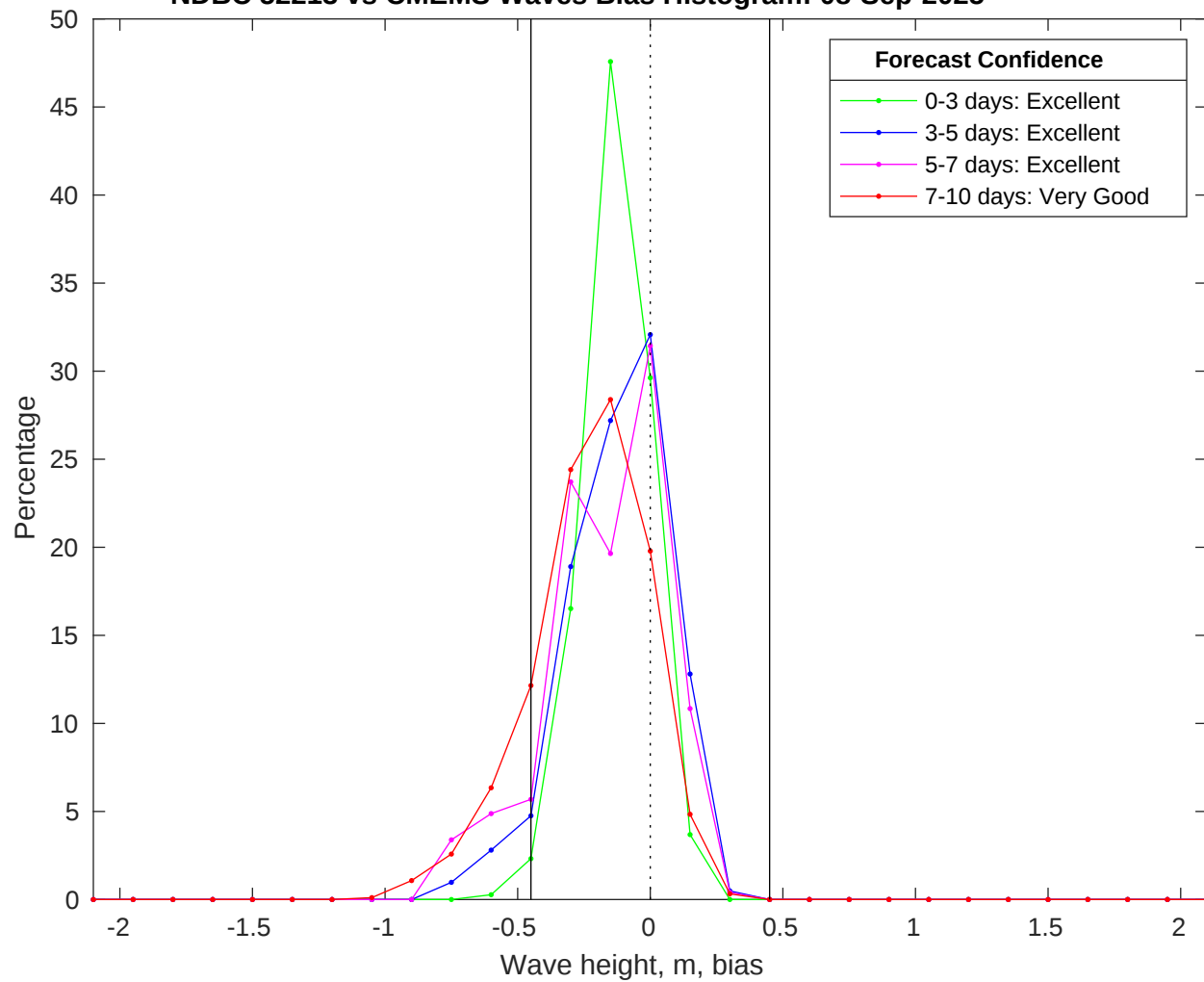
NDBC 52213 vs CMEMS Waves Bias Histogram: 08-Sep-2025
