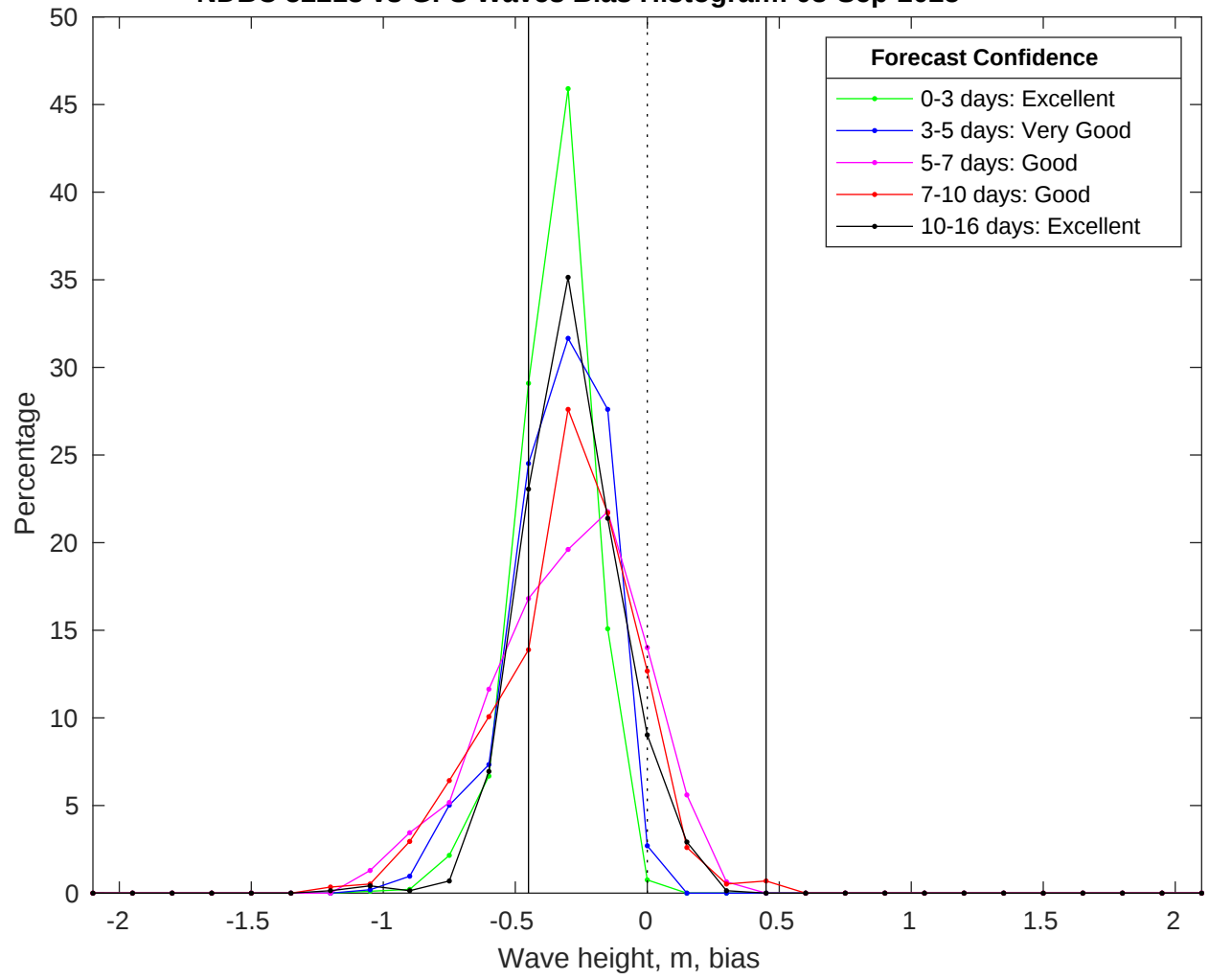
NDBC 52213 vs GFS Waves Bias Histogram: 08-Sep-2025
