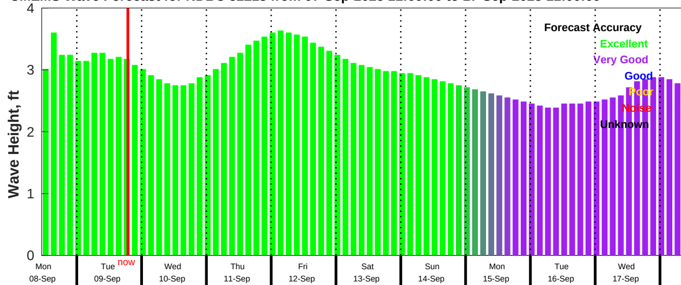
CMEMS Wave Forecast for NDBC 52213 from 07-Sep-2025 11:00:00 to 17-Sep-2025 11:00:00
