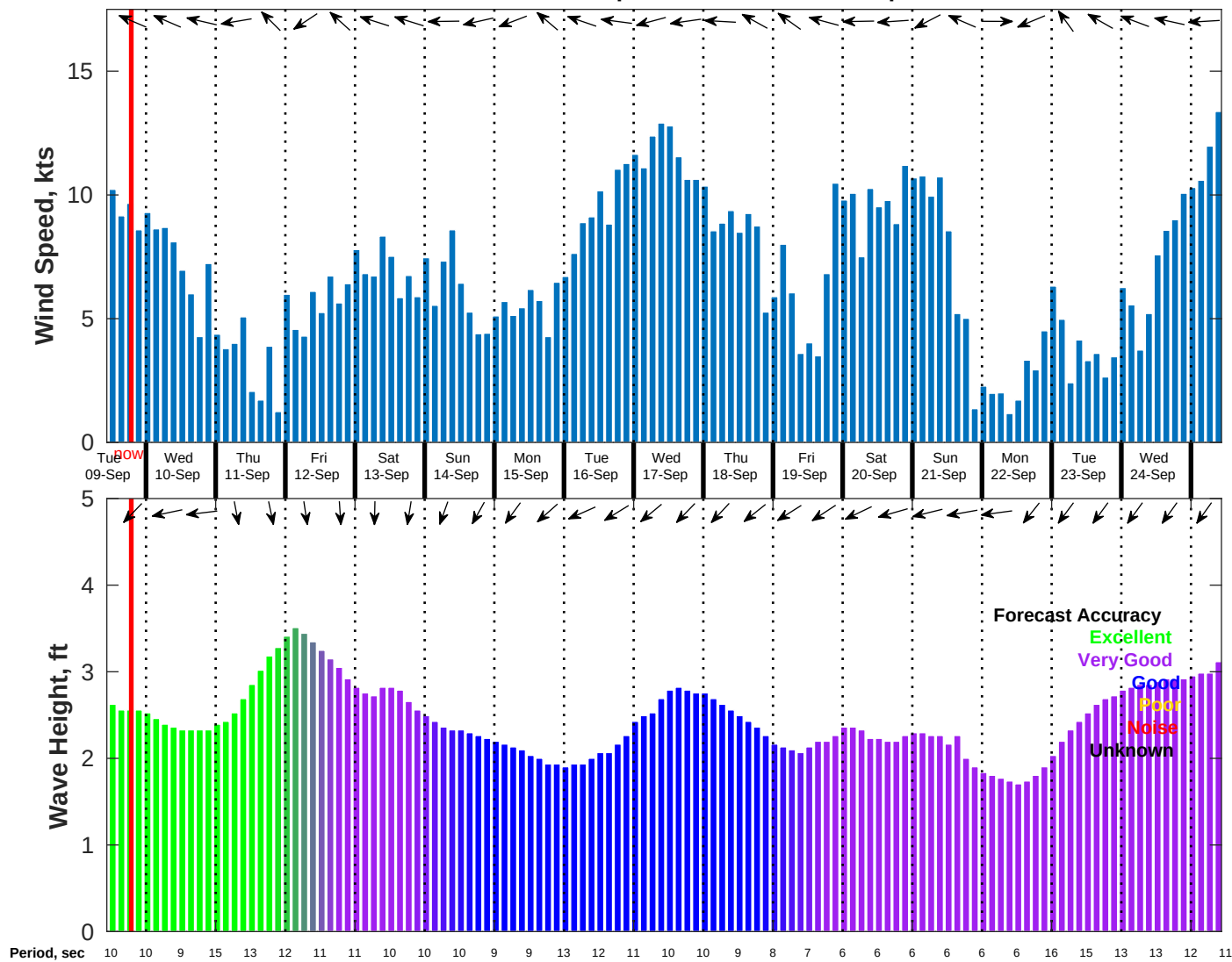
Wind & Wave Forecast for NDBC 52213 from 08-Sep-2025 11:00:00 to 24-Sep-2025 11:00:00
