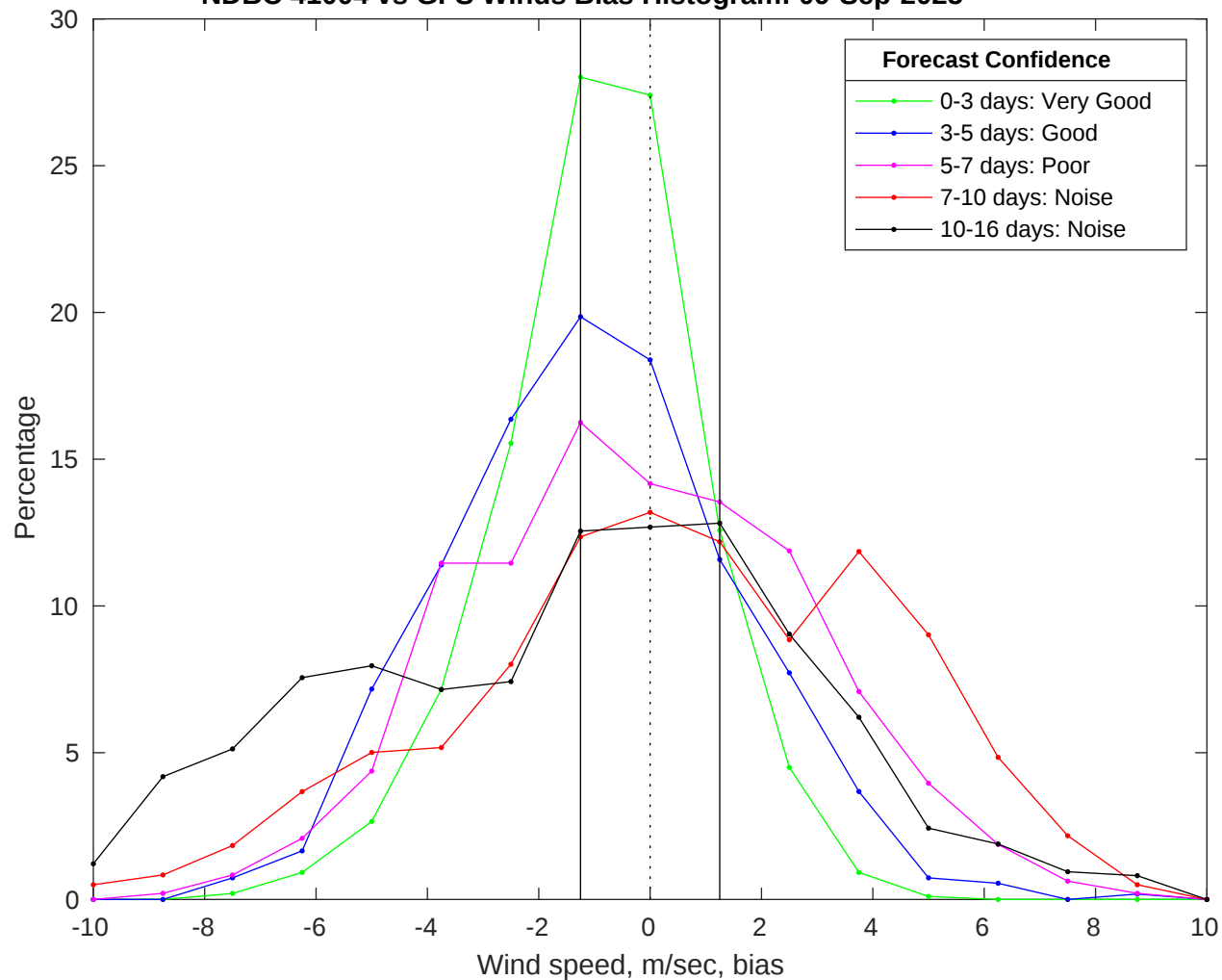
NDBC 41004 vs GFS Winds Bias Histogram: 09-Sep-2025
