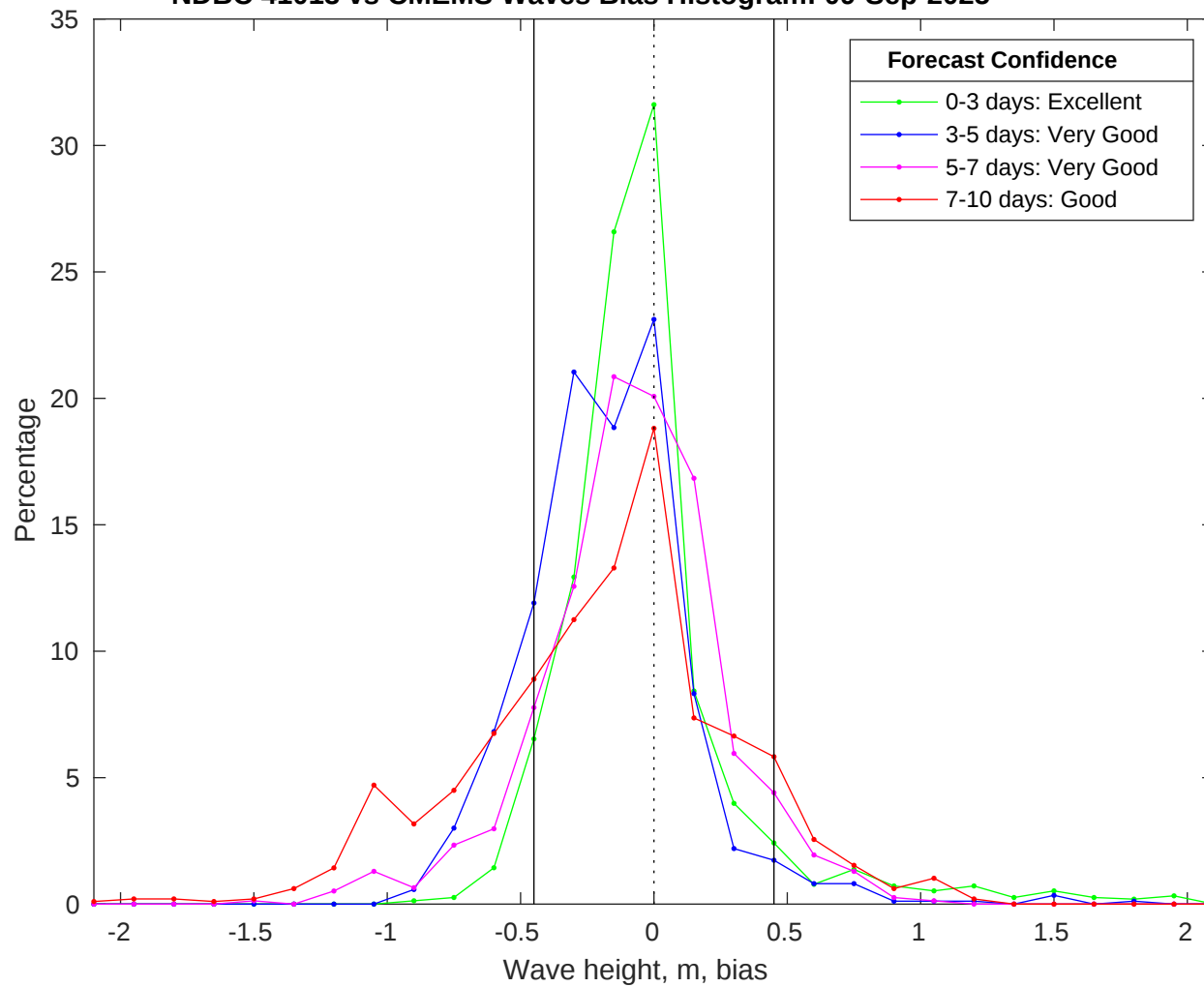
NDBC 41013 vs CMEMS Waves Bias Histogram: 09-Sep-2025
