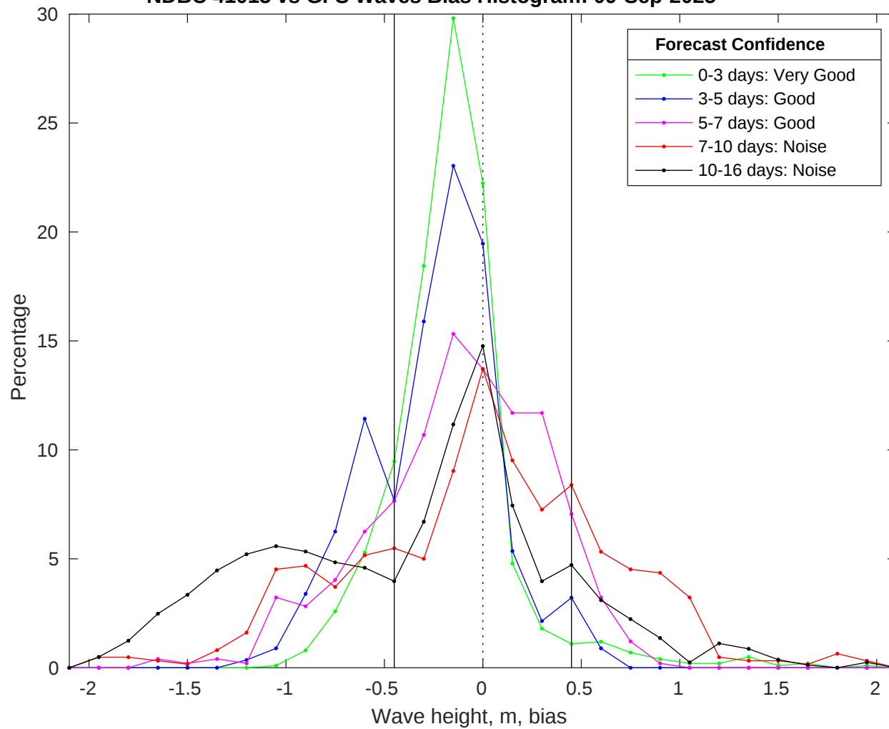
NDBC 41013 vs GFS Waves Bias Histogram: 09-Sep-2025
