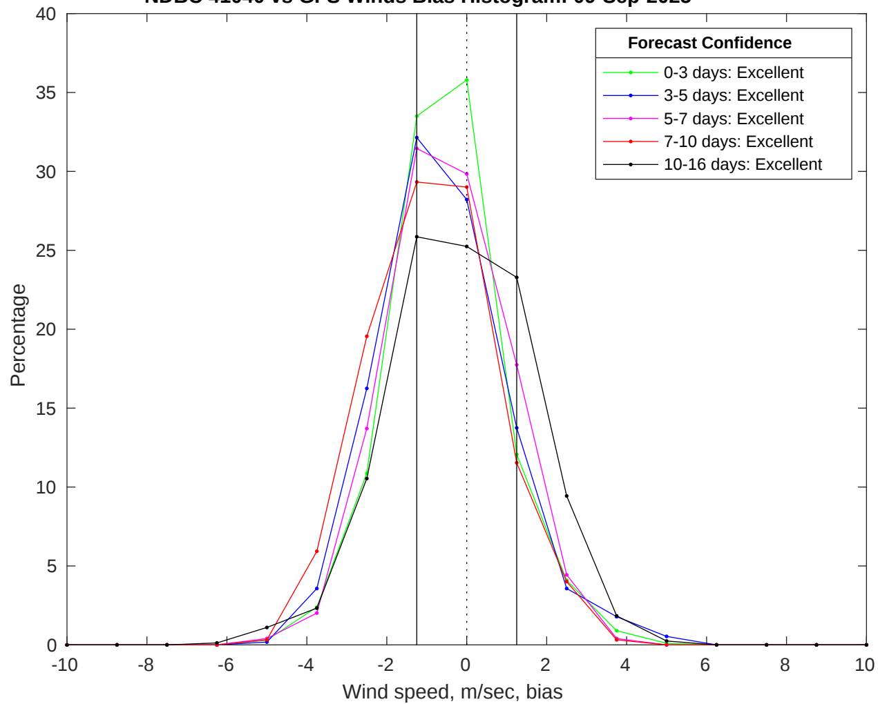
NDBC 41040 vs GFS Winds Bias Histogram: 09-Sep-2025
