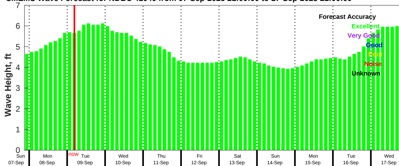
CMEMS Wave Forecast for NDBC 41040 from 07-Sep-2025 21:00:00 to 17-Sep-2025 21:00:00
