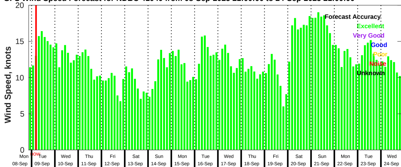
GFS Wind Speed Forecast for NDBC 41040 from 08-Sep-2025 21:00:00 to 24-Sep-2025 21:00:00
