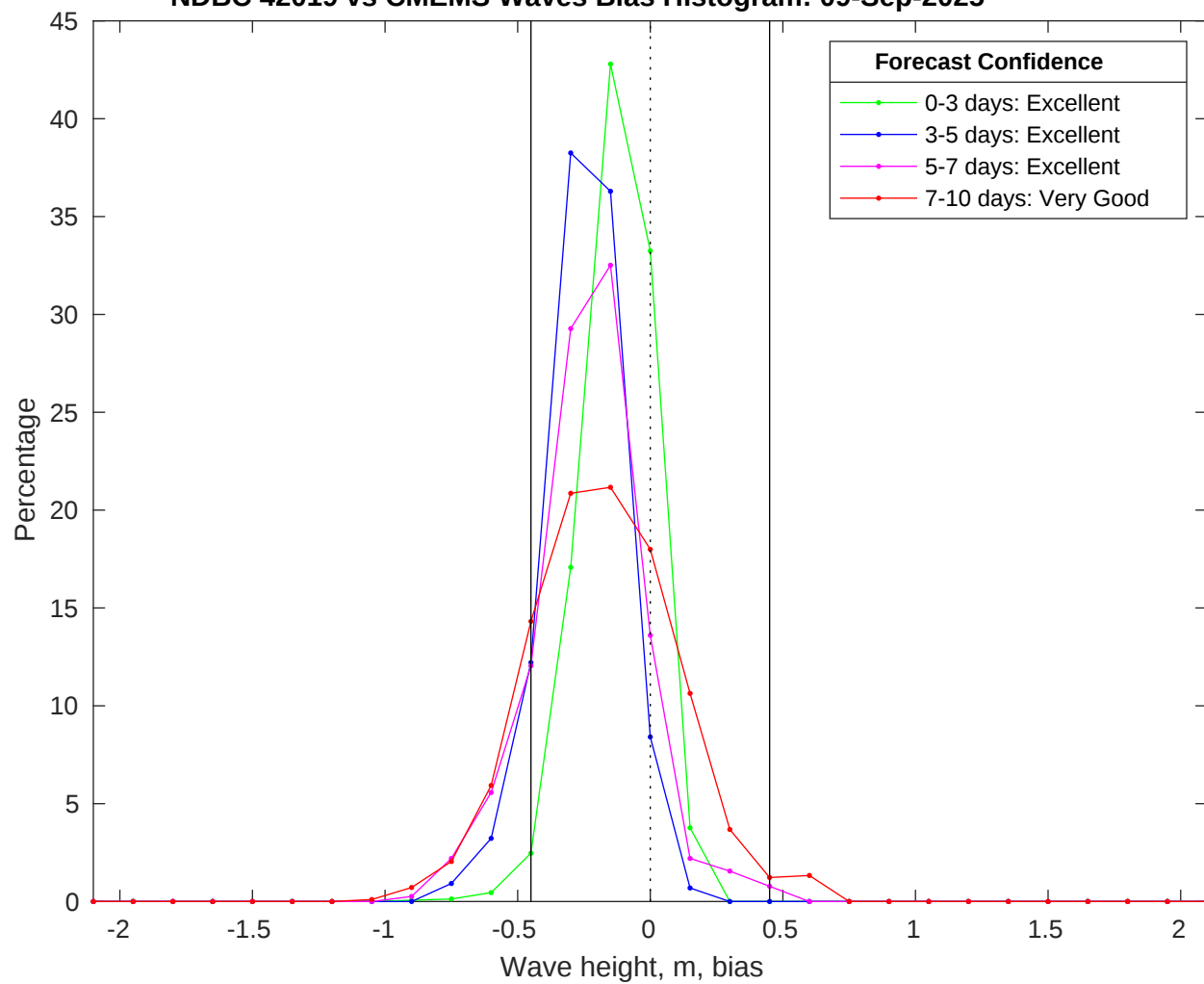
NDBC 42019 vs CMEMS Waves Bias Histogram: 09-Sep-2025
