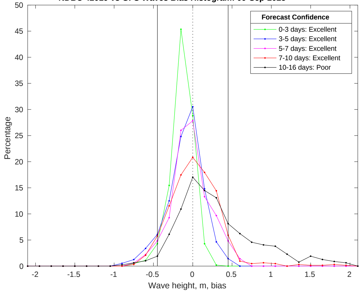
NDBC 42019 vs GFS Waves Bias Histogram: 09-Sep-2025
