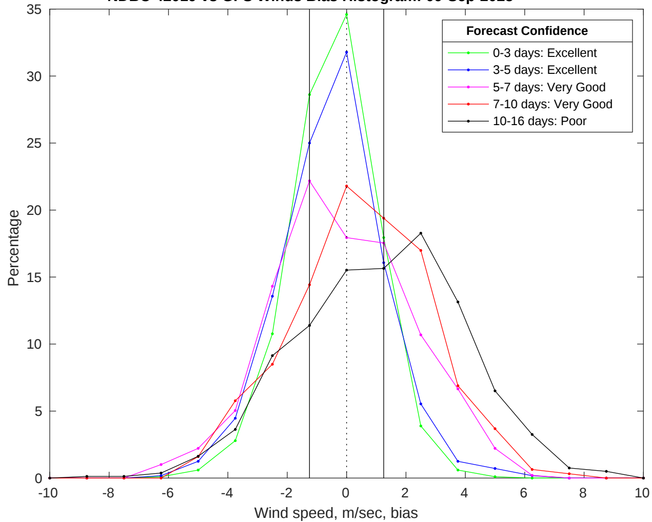
NDBC 42019 vs GFS Winds Bias Histogram: 09-Sep-2025
