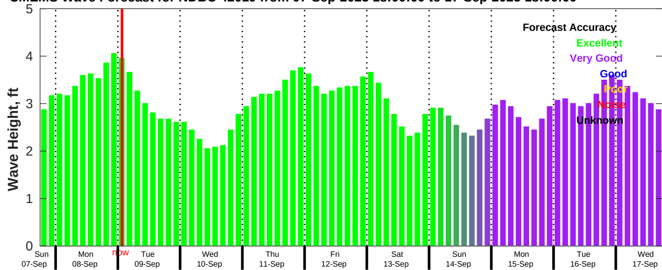
CMEMS Wave Forecast for NDBC 42019 from 07-Sep-2025 18:00:00 to 17-Sep-2025 18:00:00
