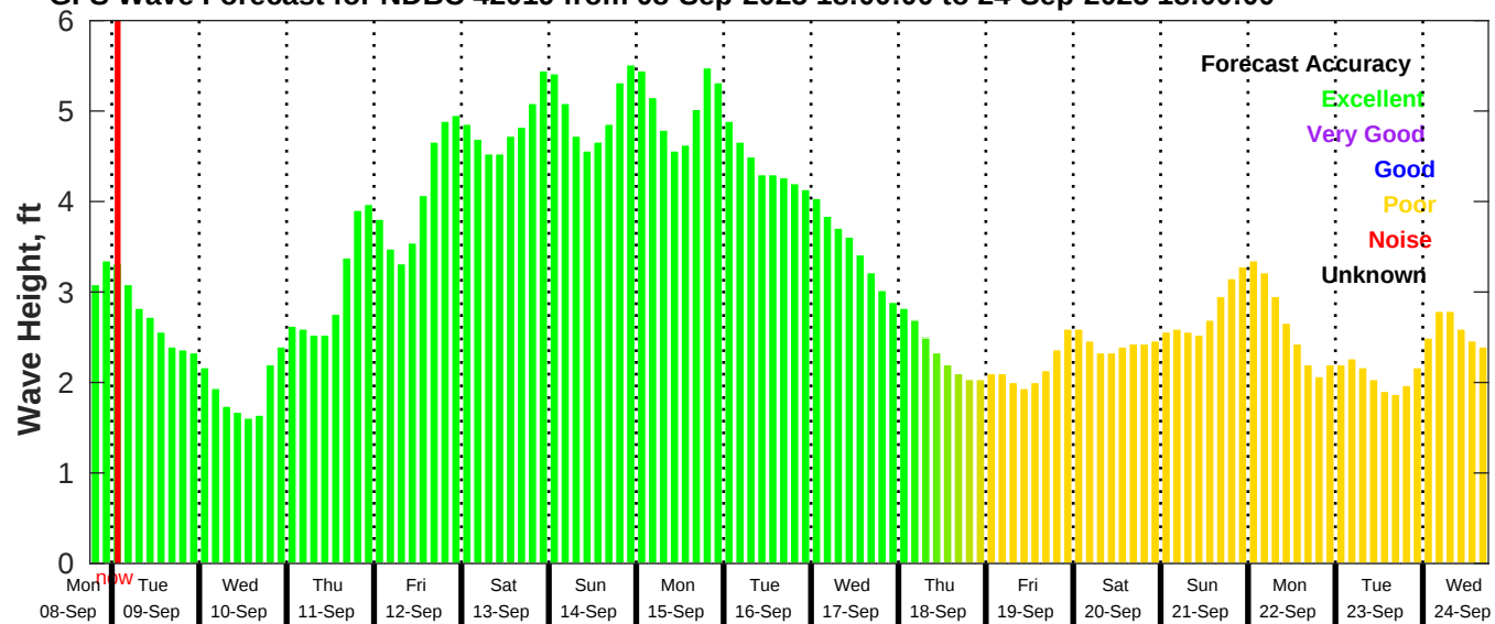
GFS Wave Forecast for NDBC 42019 from 08-Sep-2025 18:00:00 to 24-Sep-2025 18:00:00
