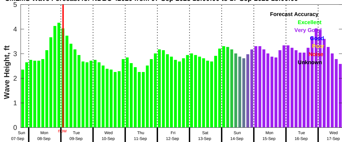
CMEMS Wave Forecast for NDBC 42020 from 07-Sep-2025 18:00:00 to 17-Sep-2025 18:00:00
