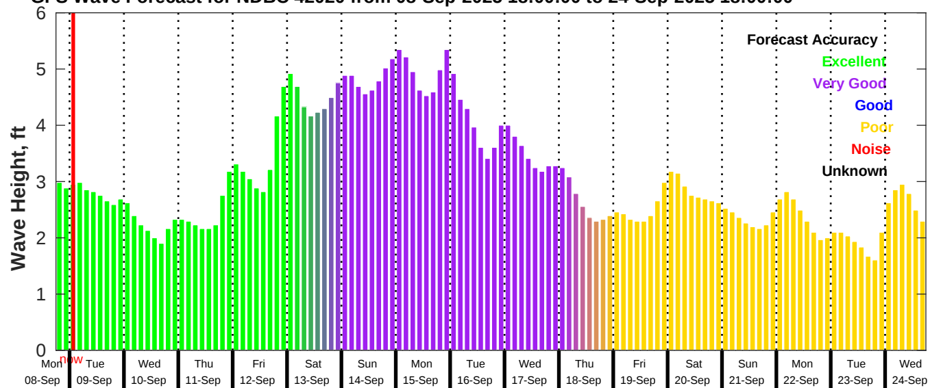
GFS Wave Forecast for NDBC 42020 from 08-Sep-2025 18:00:00 to 24-Sep-2025 18:00:00
