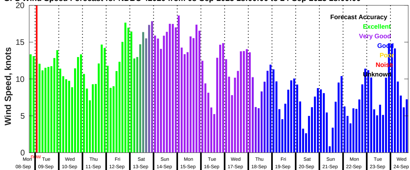
GFS Wind Speed Forecast for NDBC 42020 from 08-Sep-2025 18:00:00 to 24-Sep-2025 18:00:00
