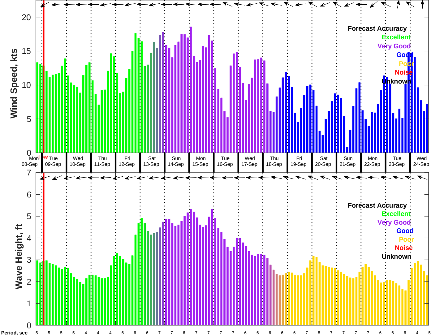
Wind & Wave Forecast for NDBC 42020 from 08-Sep-2025 18:00:00 to 24-Sep-2025 18:00:00
