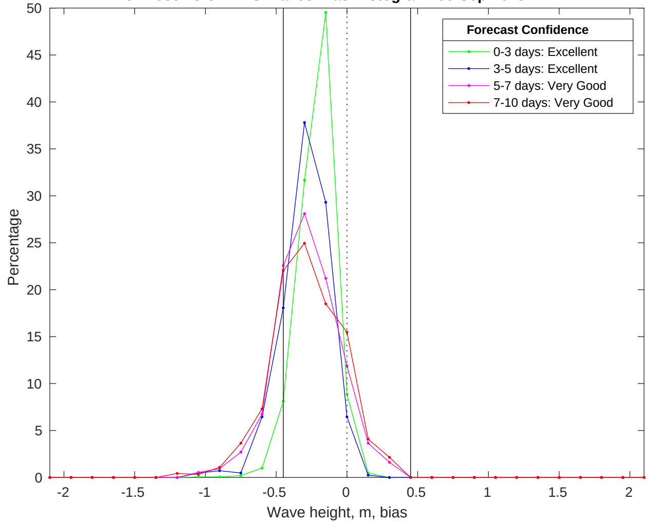
NDBC 42035 vs CMEMS Waves Bias Histogram: 09-Sep-2025
