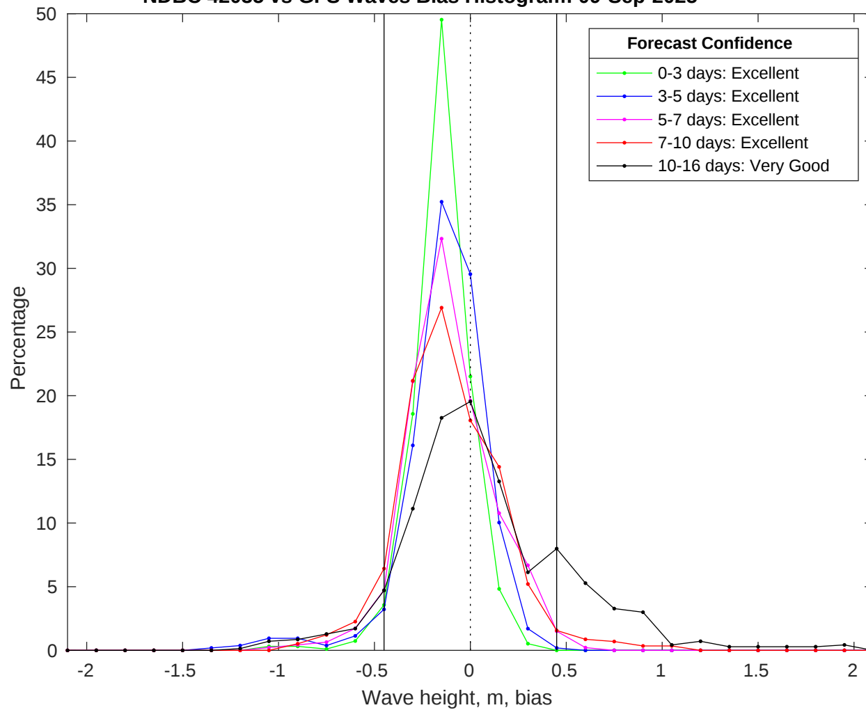
NDBC 42035 vs GFS Waves Bias Histogram: 09-Sep-2025
