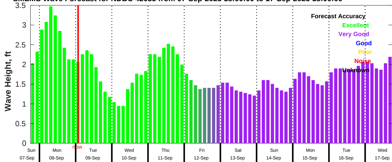
CMEMS Wave Forecast for NDBC 42035 from 07-Sep-2025 18:00:00 to 17-Sep-2025 18:00:00
