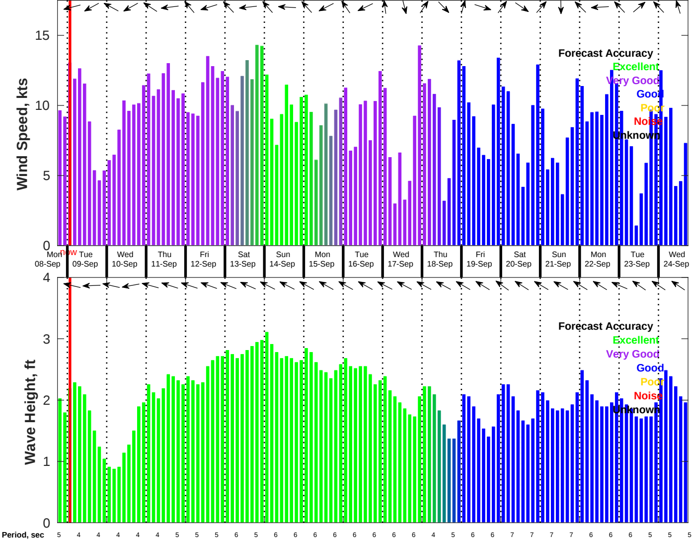
Wind & Wave Forecast for NDBC 42035 from 08-Sep-2025 18:00:00 to 24-Sep-2025 18:00:00
