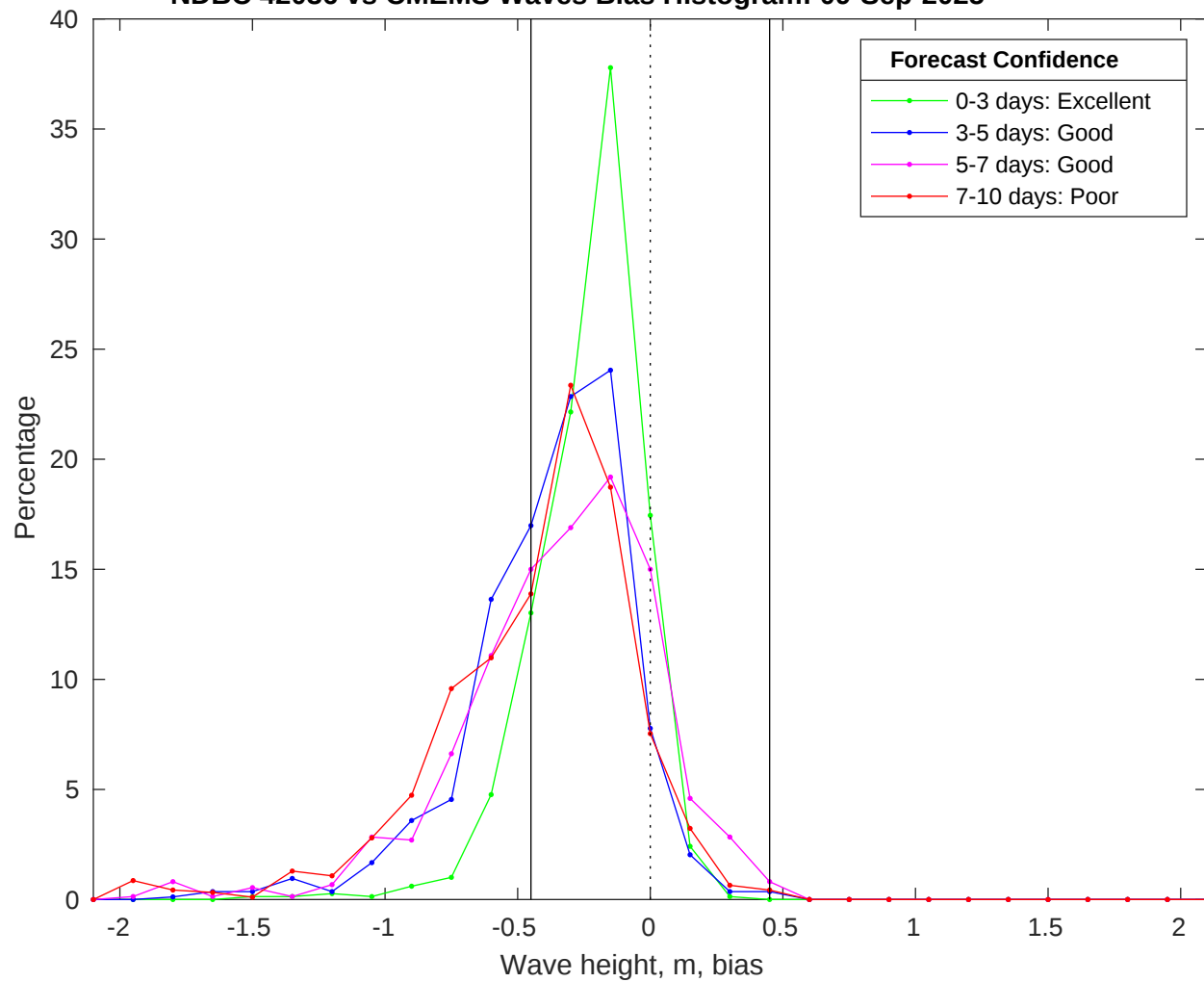
NDBC 42036 vs CMEMS Waves Bias Histogram: 09-Sep-2025
