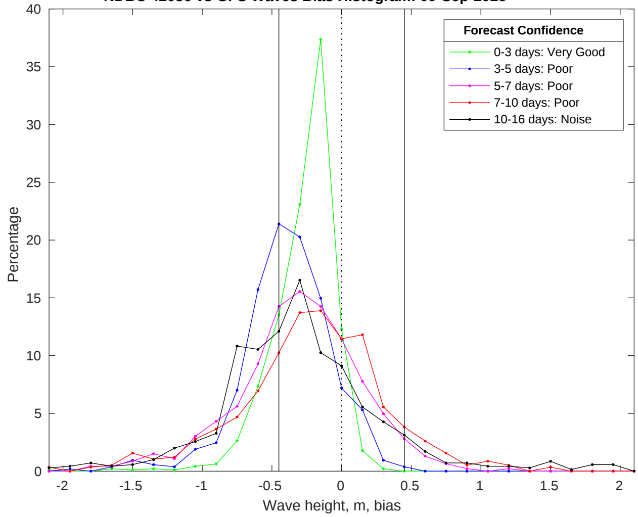
NDBC 42036 vs GFS Waves Bias Histogram: 09-Sep-2025
