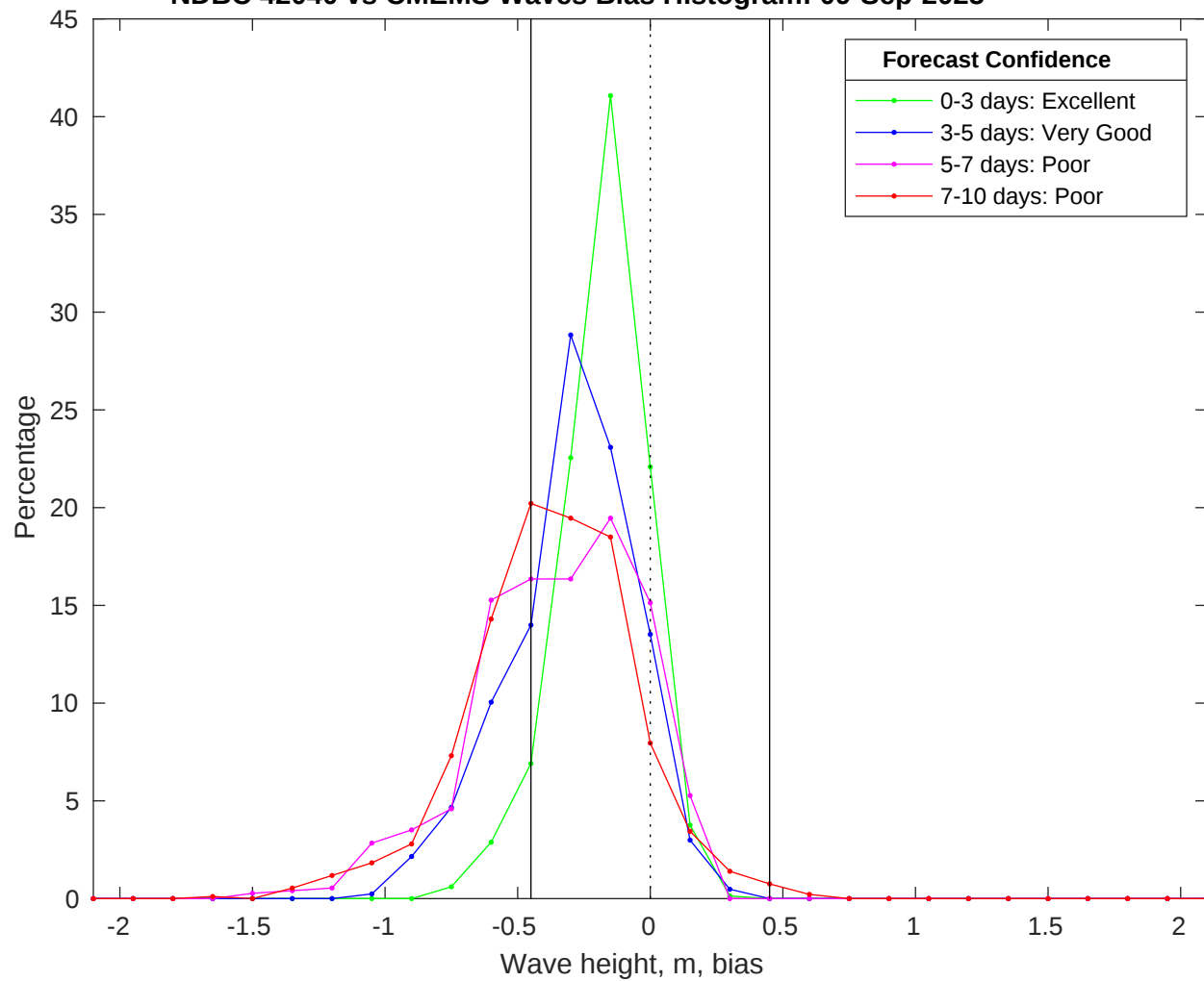
NDBC 42040 vs CMEMS Waves Bias Histogram: 09-Sep-2025
