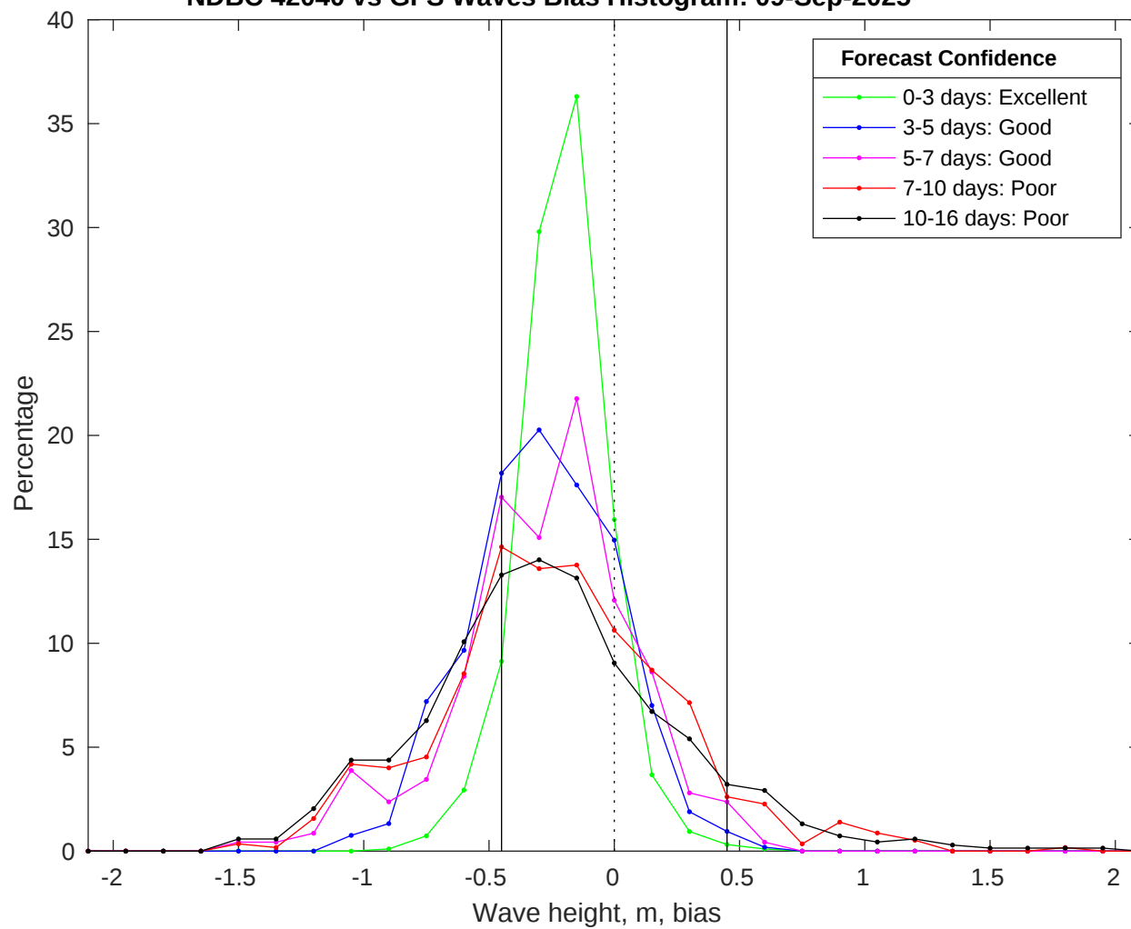
NDBC 42040 vs GFS Waves Bias Histogram: 09-Sep-2025
