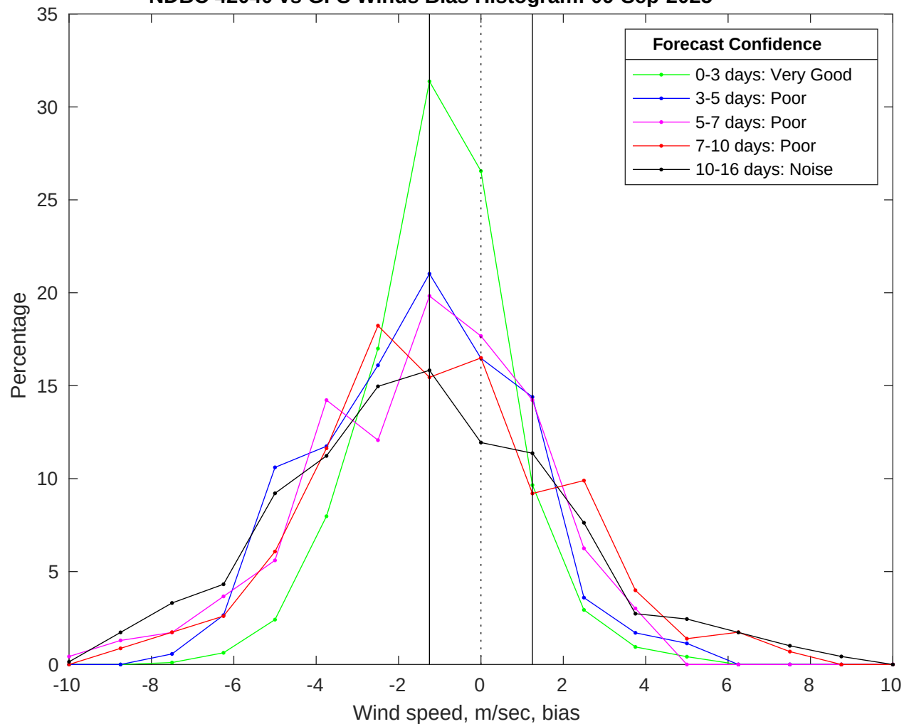
NDBC 42040 vs GFS Winds Bias Histogram: 09-Sep-2025
